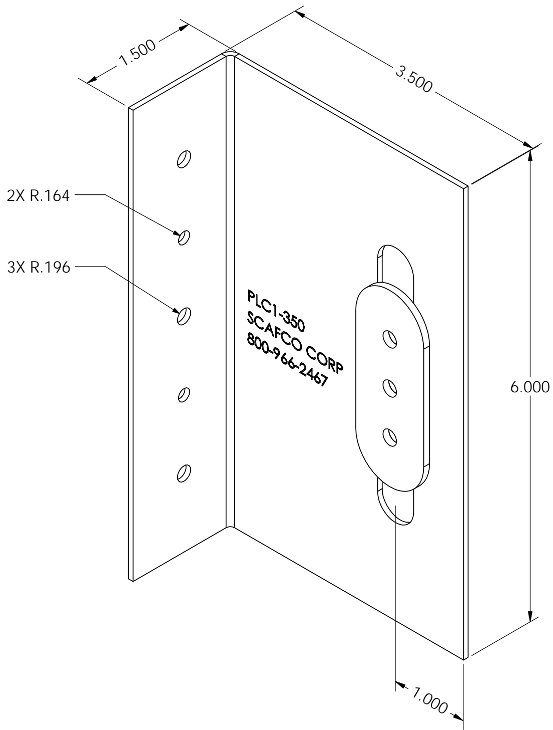
PLC1-350 DEFLECTION SLIDE CLIP
