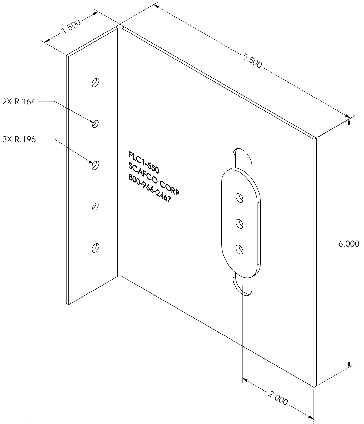
PLC1-550 DEFLECTION SLIDE CLIP
